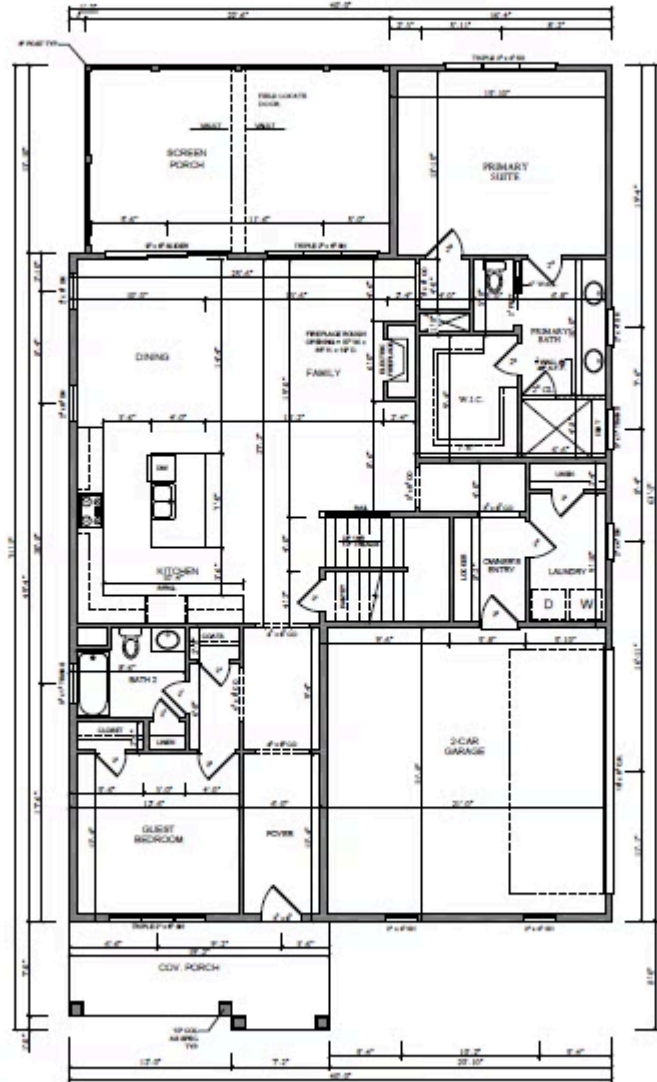
FIRST FLOOR PLAN NOT TO SCALE REVISIONS: 1/1/11
