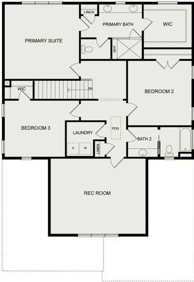
THE BELLAMY- CRAFTSMAN SECOND FLOOR PLAN
