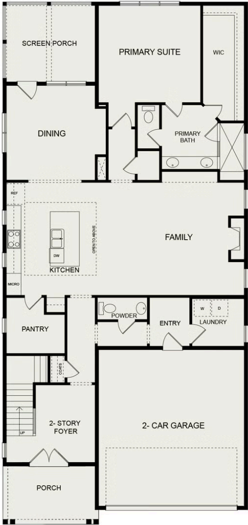
THE LEIGHTON- CAPE COD FIRST FLOOR PLAN
