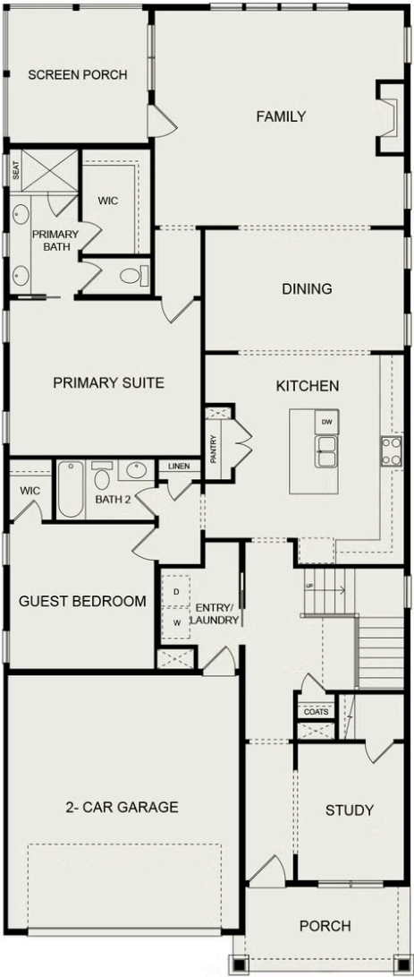
THE ROSEMARY-CRAFTSMAN FIRST FLOOR PLAN
